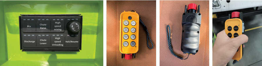
2.Remote control: 1) High speed mixing/discharge. 2) Barrel can maintain a constant speed, can be controlled by remote.
